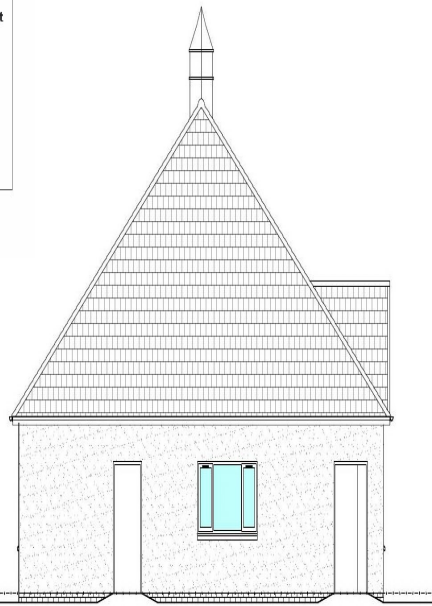
south (side) elevation
